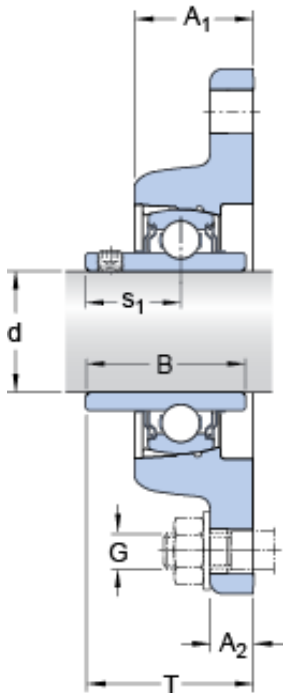
FYT 35 TF/VA201 Bearing 2D drawings and 3D CAD models
